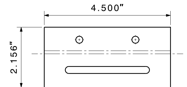
Flat Pattern Scale 1:2
