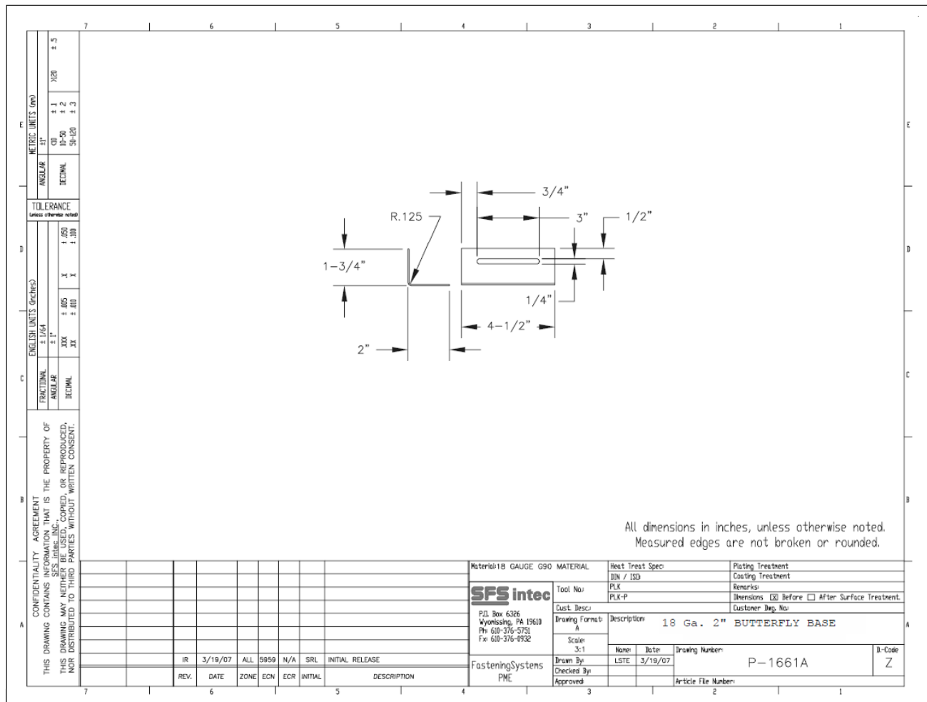
Drawing No. 2 Clip Base Details
