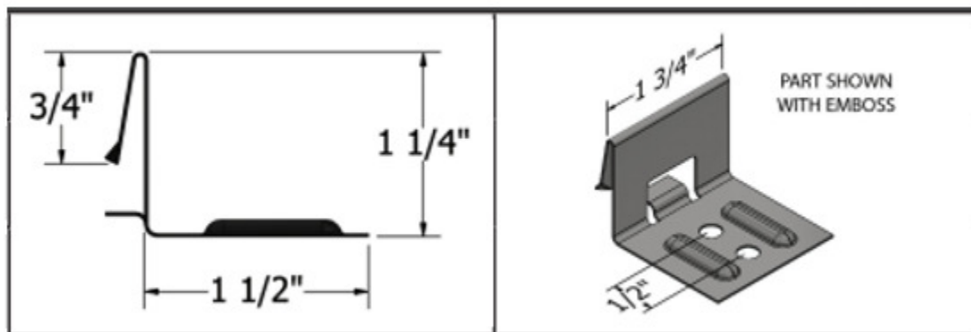
Drawing No. 2 Clip Details
